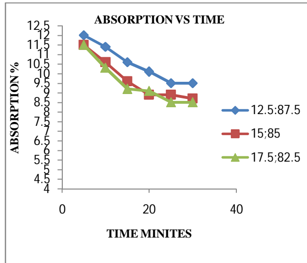
Figure 6. Water Absorption of Aggregates
